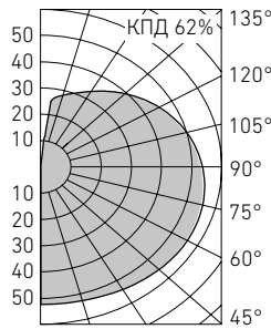
NBL 70 E40 sphere opal
