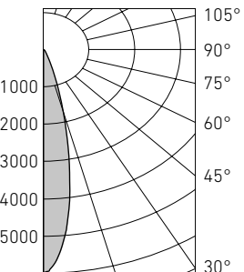
WALLWASH R LED 30 (15)
