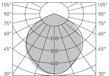
ECO FLOOD LED 30
