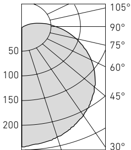
DAMIN LED 40
