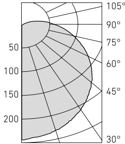
DAMIN L LED 40
