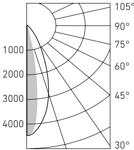
WASHLINE LED 18 (15x30)
