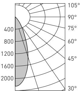
WALLWASH LED 45 (30)
