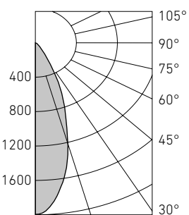
WALLWASH R LED 30 (30)
